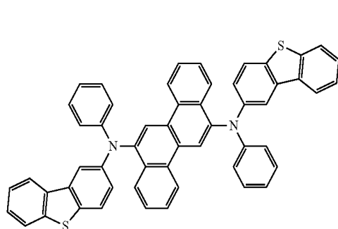
-continued FD8
