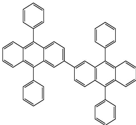
Compound FD(3)
