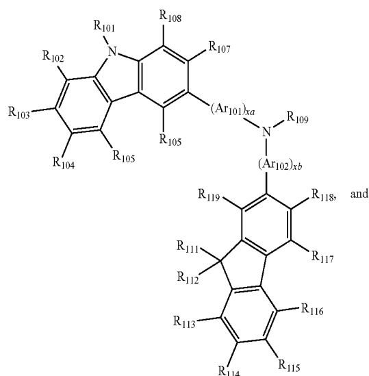
Formula 201
