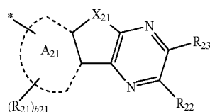
Formula 3-1
