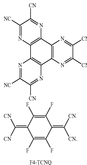
F4-TCNQ
