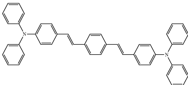
Compound FD(8)
