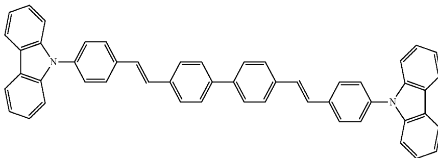
Compound FD(3)
