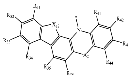
Formula 13-1
