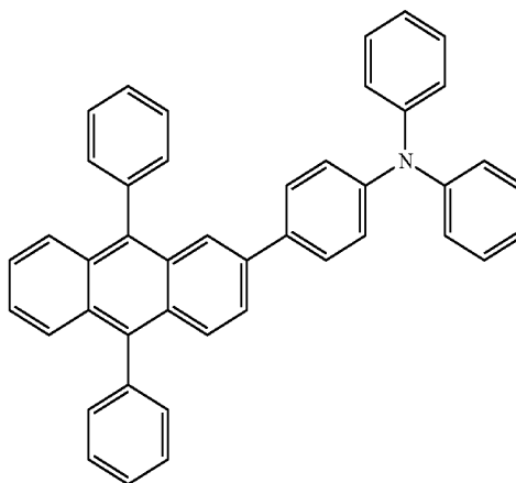
Compound FD(4)
