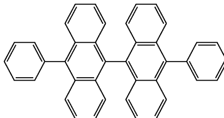
Compound FD(13)
