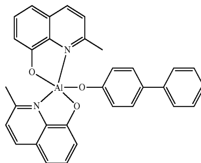
BAQ
