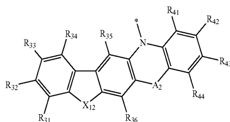
Formula 13-4
