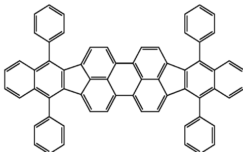
Compound FD(10)
